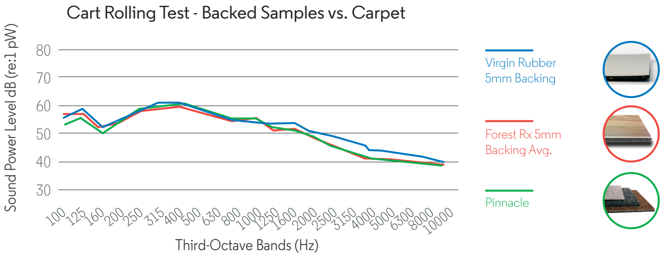
Cart rolling test results for ECOsurfaces’ Forest Rx sheet vinyl (5mm backing), ECOsurfaces’ virgin rubber (5mm backing), and Pinnacle 5mm rubber backed commercial grade carpet.
