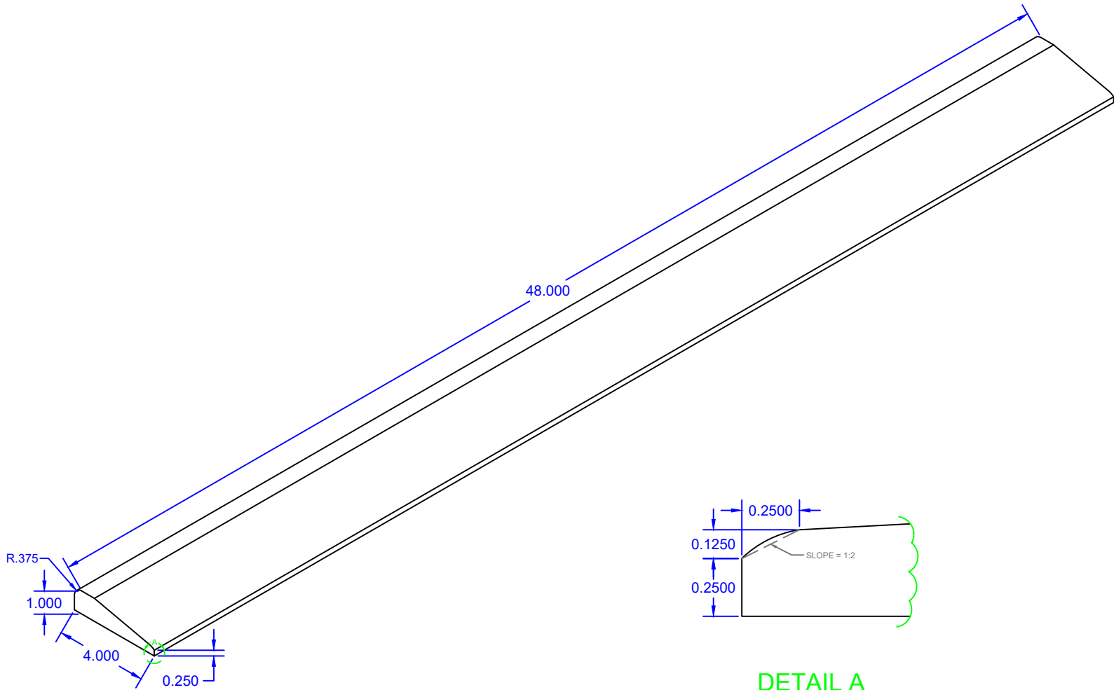
DETAIL A
